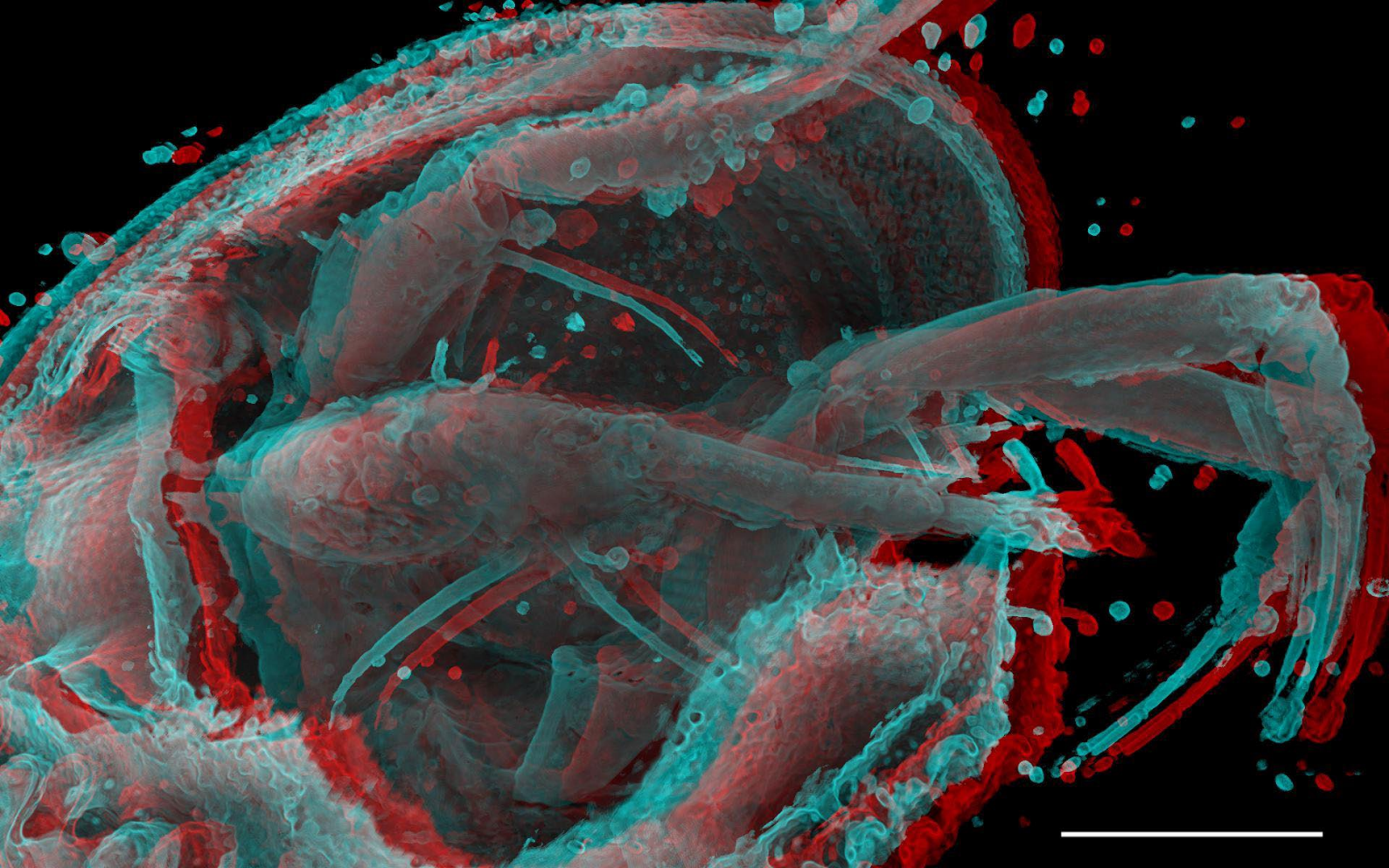
Figure S2. View inside the anterior part of the carapace of the adult male Myanmarcypris hui specimen (BA19005-1). Data visualization by volume rendering in Drishti in red-cyan. In this mode the investigation of appendages and chaetotaxy were carried out by using tools such as rotate, zoom, clip, and carve, and by modifying the two-dimensional transfer functions.
